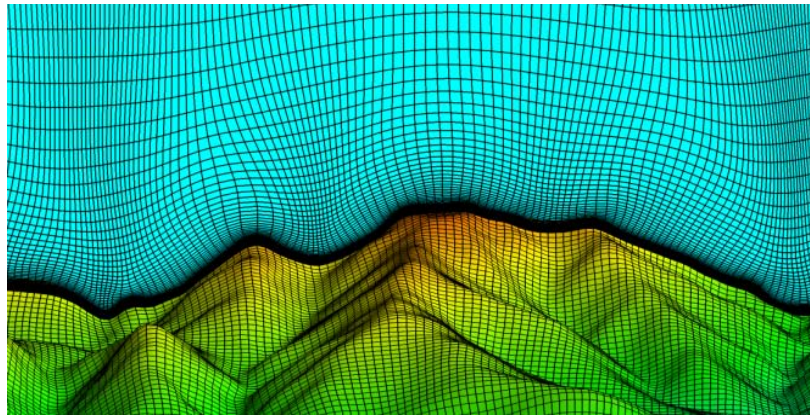
Figure 1: Example of a computational mesh for terrain CFD simulation.
